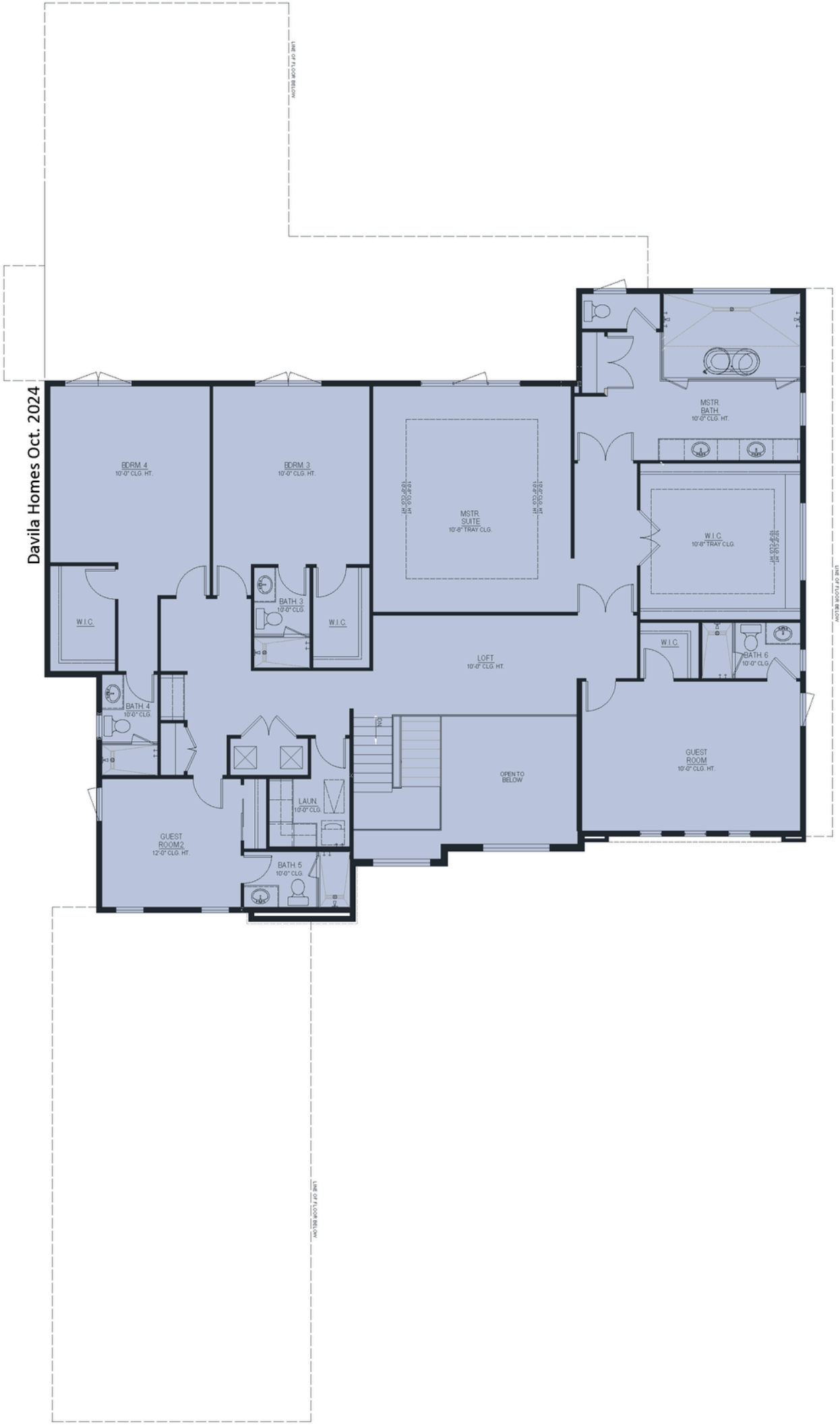
SECOND FLOOR
